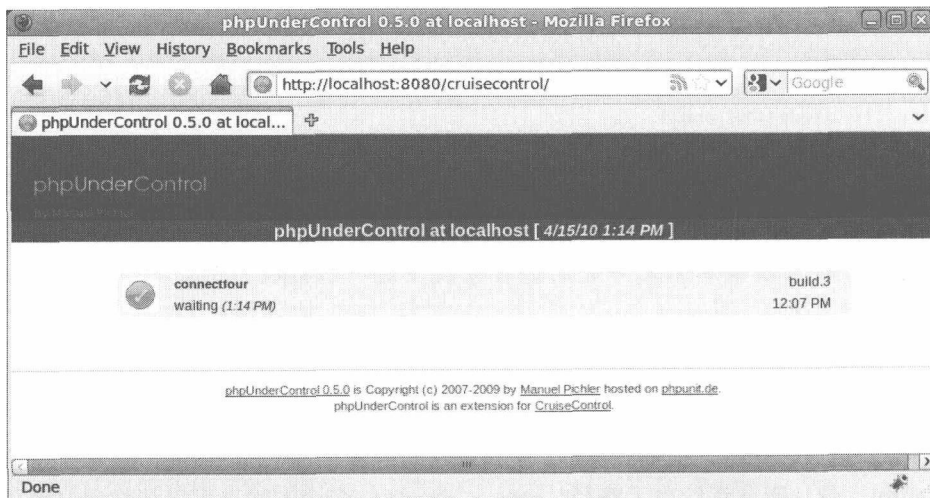
图20-5 phpUnderControl
